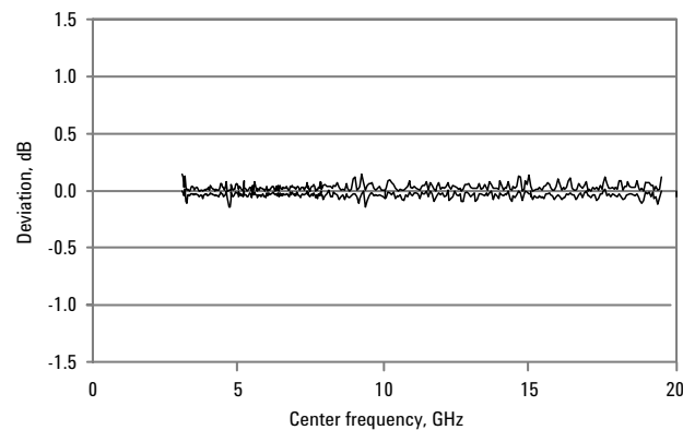
Figure 5. Nominal peak positive and negative amplitude deviation after calibration (preselector bypassed, 64 MHz bandwidth)
