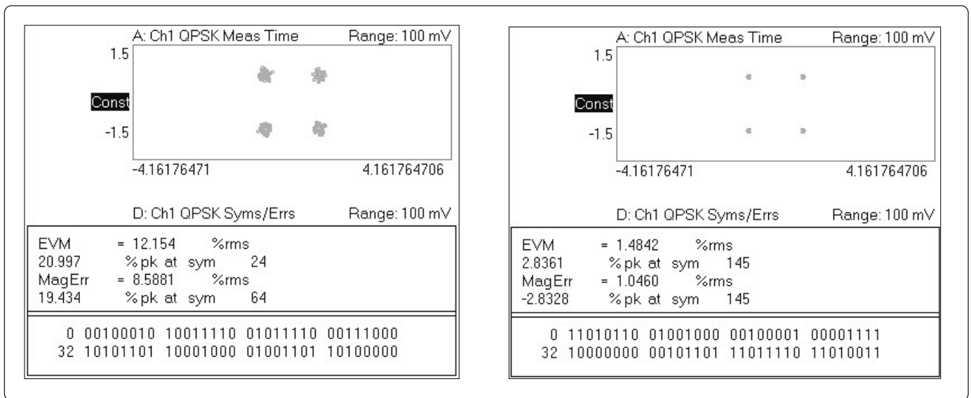
Figure 14. QPSK constellation and EVM summary table before (left image) and after (right image) extended calibration 1
