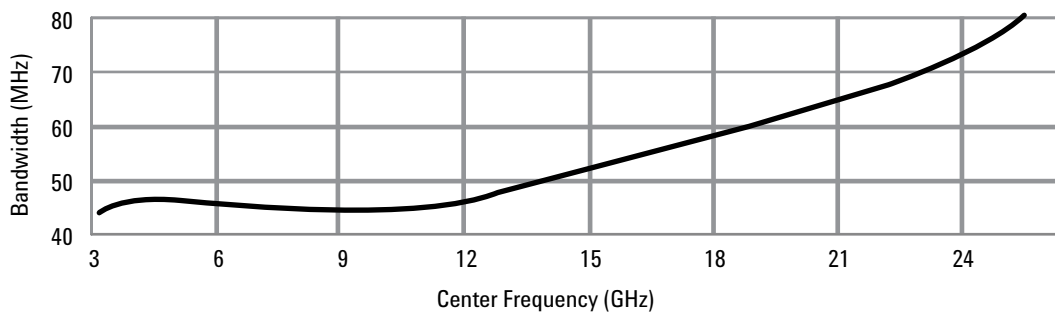
Figure 9. PSA Option 122 nominal IF bandwidth (–4 dB) versus center frequency, CF > 3.05 GHz, without Option 123. For Option 140, the IF response is identical over –18 MHz to +18 MHz.
