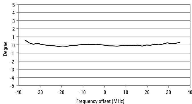
Figure 7. Phase deviation after calibration, 72 MHz span at 18.1 GHz (preselector bypassed)
