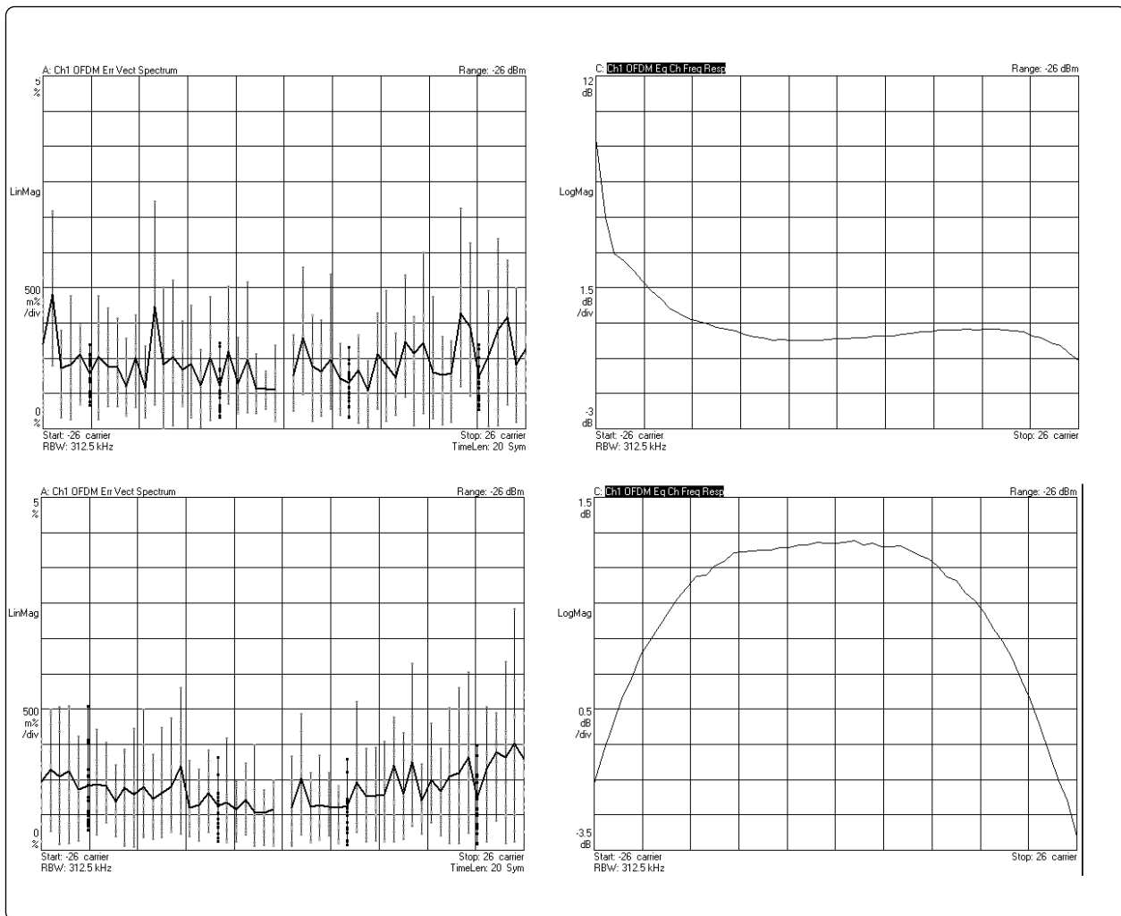
Figure 12. OFDM error vector spectrum and channel response before (top) and after (bottom) extended calibration 1
